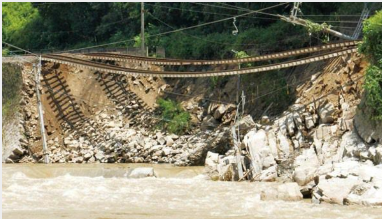
Damaged Railway by torrential rain in July, 2018 in Higashihiroshima city
